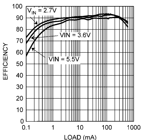
Efficiency vs. Output Current, V_{OUT1} = 1.2V 20167381
